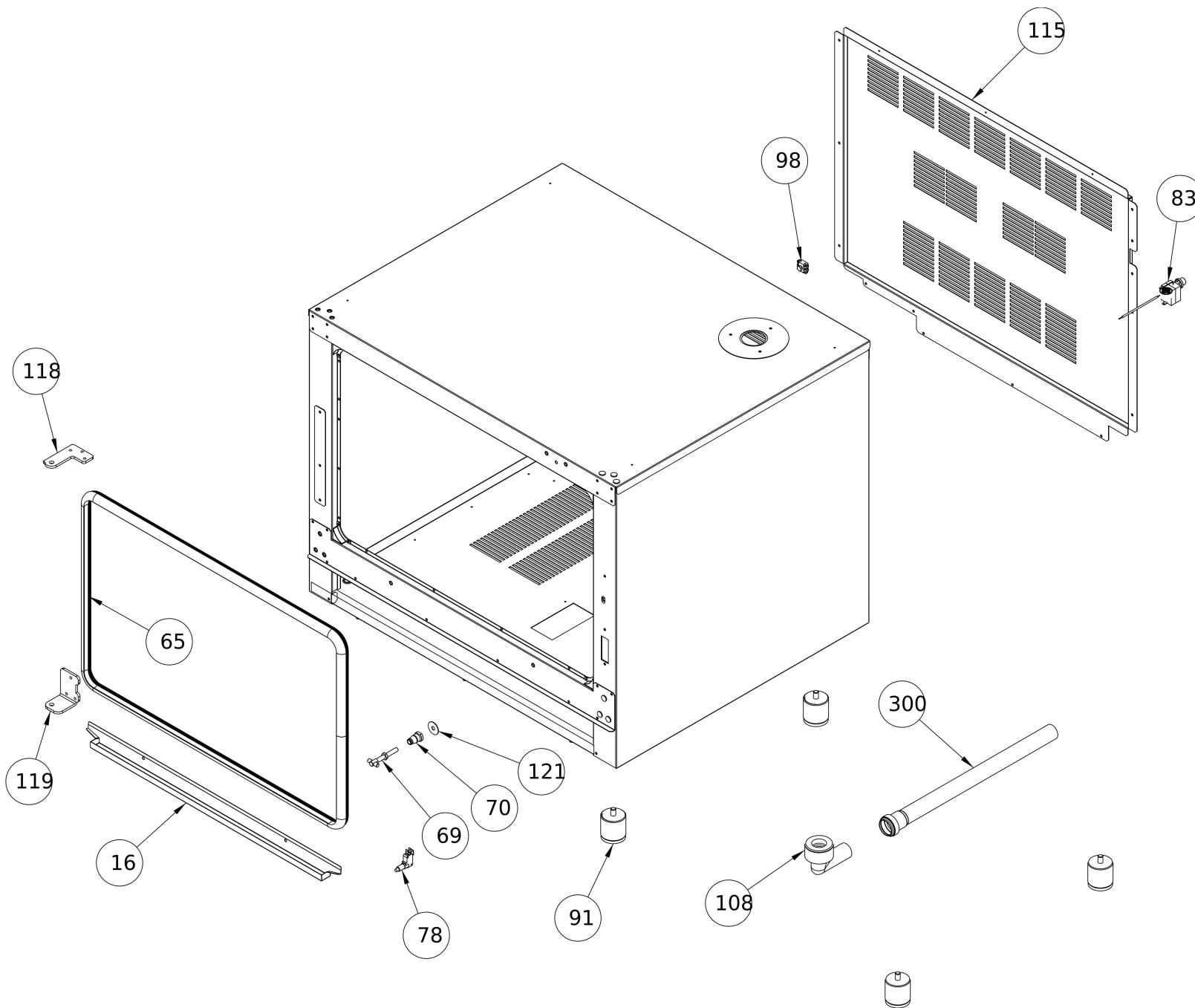
Oven body
