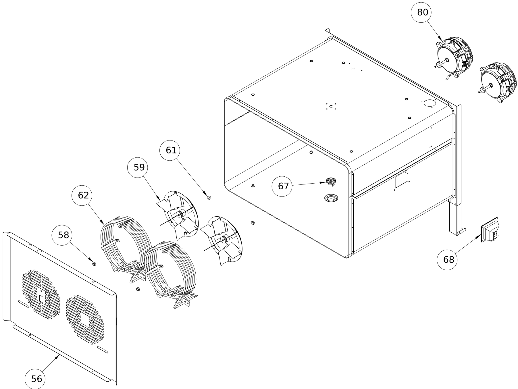
Cooking chamber
